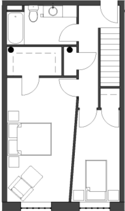
TOWNHOUSE Lower Floor 3/16"=1'-0"
