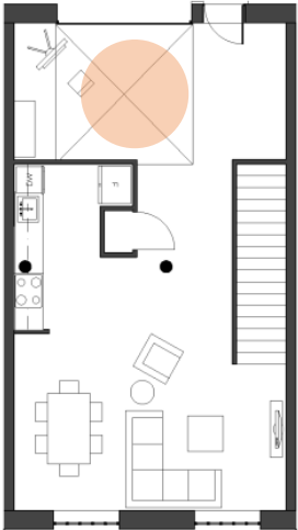
LIVE/SELL Upper Floor 3/16"=1'-0"
