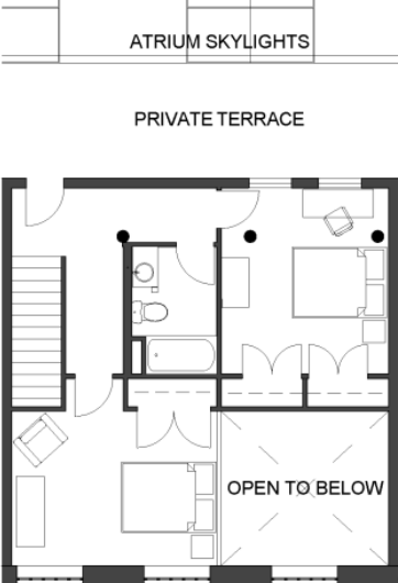
UPPER LEVEL TOWNHOUSE Upper Floor 3/16"=1'-0"
