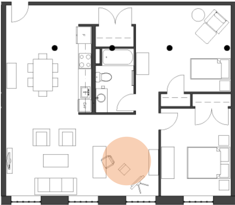
2 BEDROOM FLAT 3/16"=1'-0"
